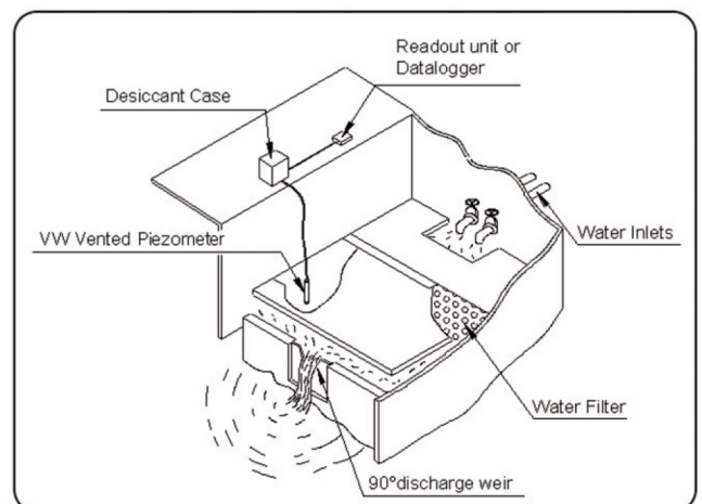
[Installation of VW vented piezometer]
